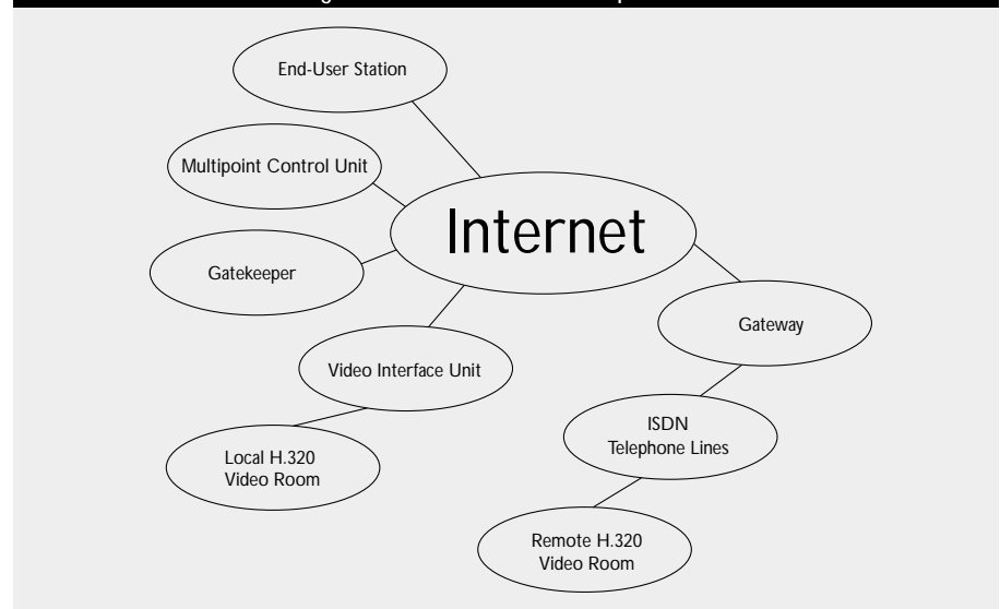
Figure 3: H.323 Video Components
